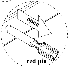
Drawer Rail Assemble Detail
