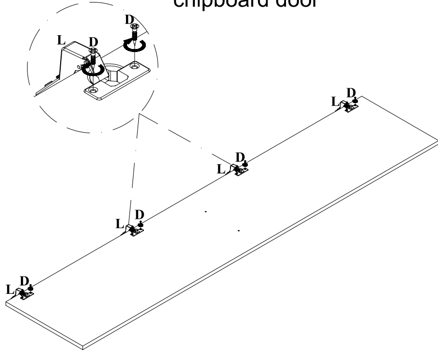
"chipboard door"
